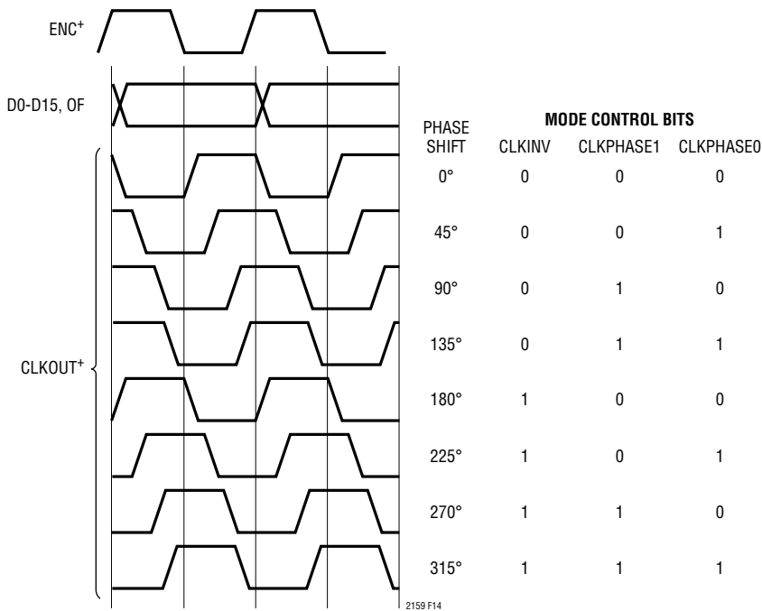
Figure 14. Phase-Shifting CLKOUT
